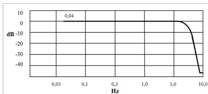
Frequenzgang KS22-I
