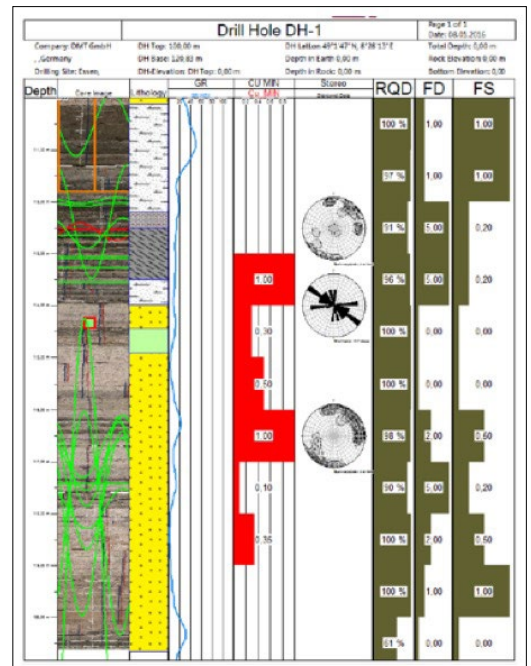
Composite log with grade and structural / geotechnical analysis structures
